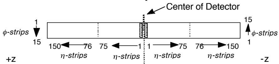
Figure 19: Relationship between the EMC modules on the +z and -z side. The labels for the shower max are also shown. The view on the shower max is from the perspective a person looking down from outside the detector.
