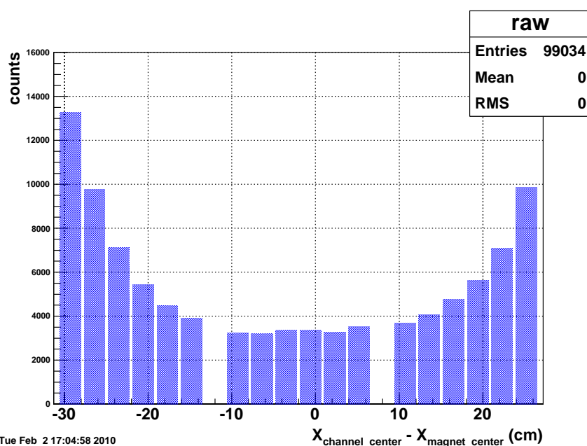
Figure 15. The MTD raw hits distribution along the \phi direction in 200 GeV Au+Au collisions in year 2010. There are three LMRPC modules, 18 strips in total. The strip size is 87 \times 2.5 \text{ cm}^2 .
