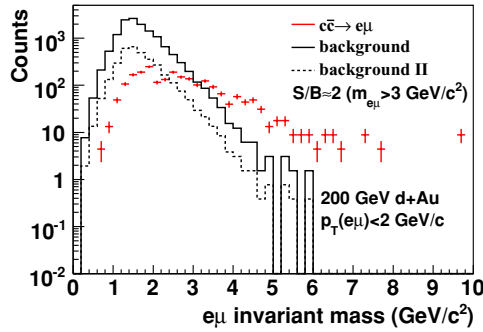
Figure 11. The expected electron–muon correlation from charm pair production and from random background in d+Au collisions. The statistics shown are equivalent to 2 billion minbias d+Au collisions.
