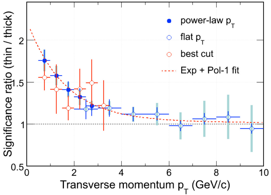
Figure 4: Impact of PXL thickness on signal significance as a function of p_T . The different symbols represent different p_T shapes and/or optimized cuts, as labeled.
