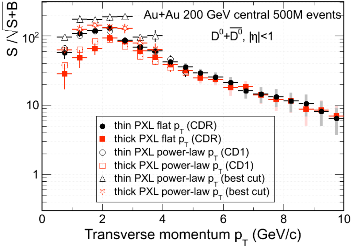
Figure 2: Signal significance as a function of p_T . Filled/open circles/squares shows the change in significance due to thickness (thin/thick) for flat/realistic spectral shape. Open triangle/stars show a new result, the signal significance for thin/thick after a careful cut optimization was performed in the lower p_T region.
