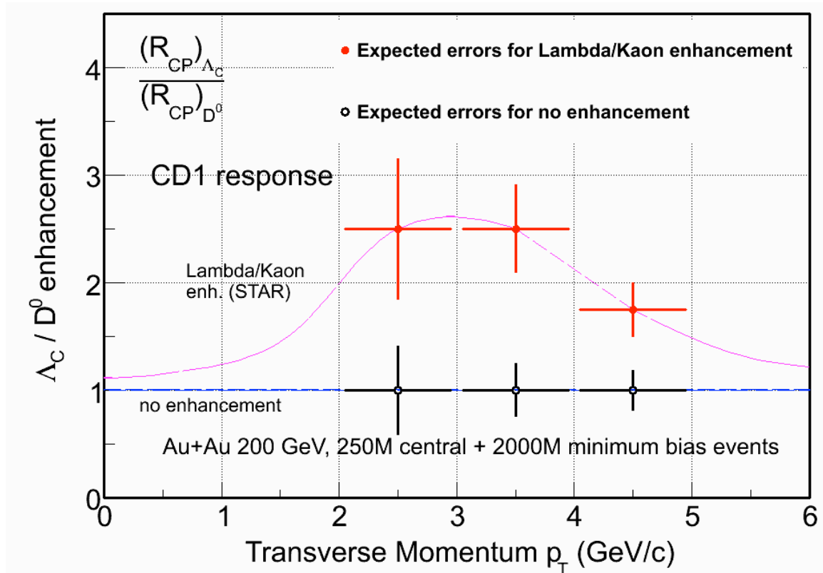
Figure 7: Expected statistical errors of the ratio of \Lambda_c to D^0 production for different assumptions about the production mechanism.
