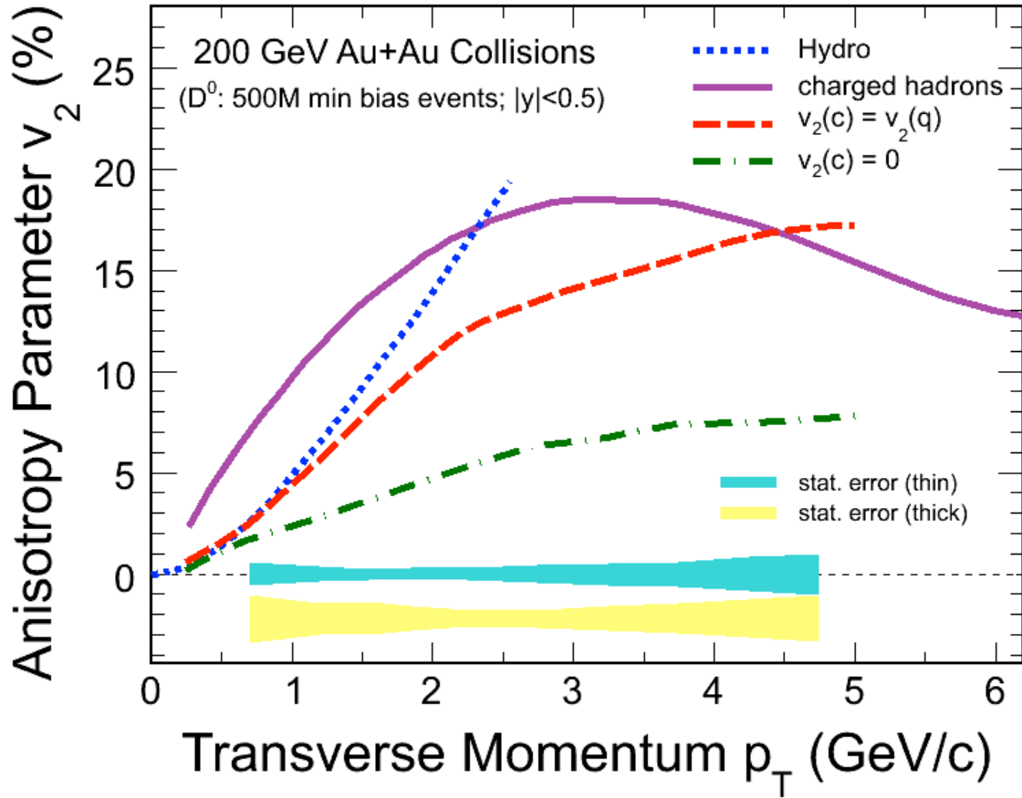
Figure 1: Elliptic flow ( v_2 ) vs p_T in Au+Au collisions at 200 GeV. The purple curve shows the measured value for charged hadrons. The red and the green curves show calculations from Ref [1] for the limiting cases that the charm quark flows like the light quarks and that the charm quark does not flow. The cyan band indicates the statistical error that can be achieved with 500 M minimum bias events for the thin detector configuration and the yellow band is for the thick configuration.
