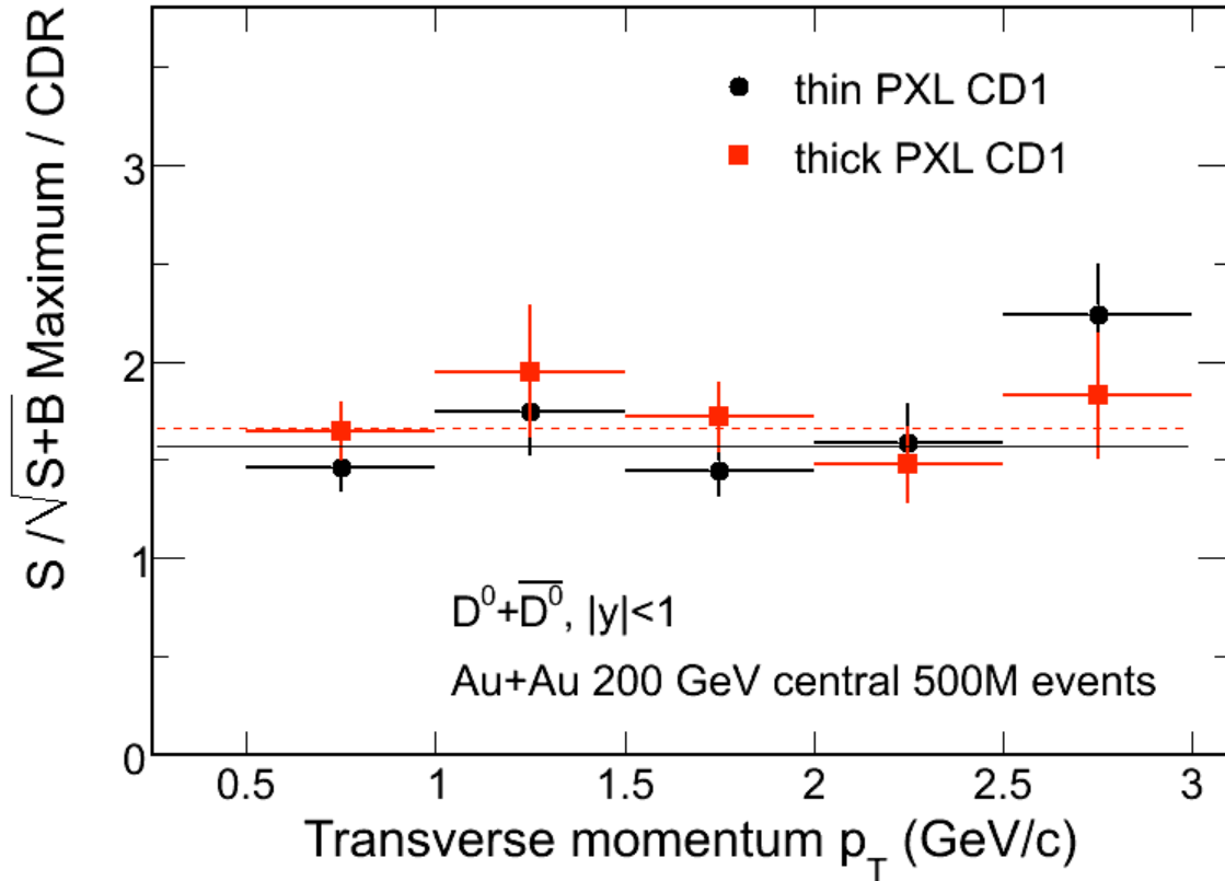
Figure 5: Signal significance gain as a function of p_T after cut optimization for thin (black symbols) and thick (red symbols).
