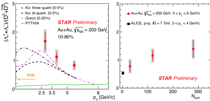
Figure 2. The \Lambda_c^\pm/D^0 ratio as a function of p_T for 10-80% centrality class (left) and as a function of N_{part} for 3 < p_T < 6 GeV/c (right), in Au+Au collisions at \sqrt{s_{NN}} = 200 GeV. The error bars and gray bands represent statistical and systematic uncertainties, respectively.
