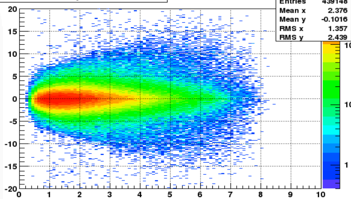
pull XY versus 1/p for No. HFT = 3
