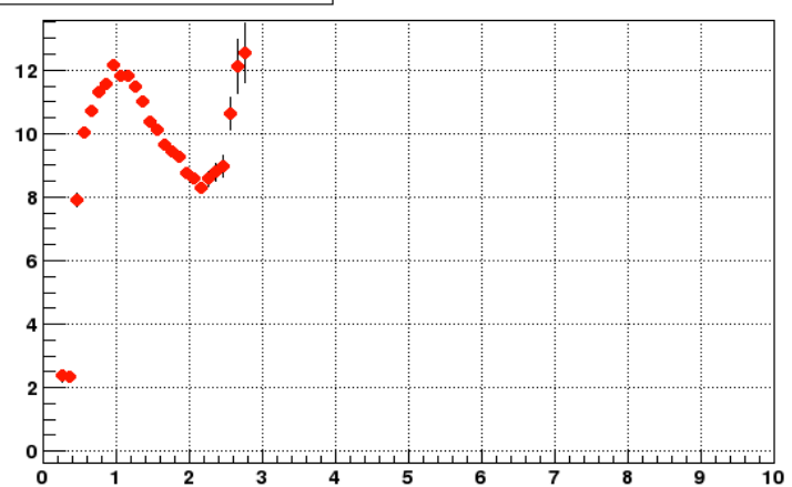
Fitted value of par[2]=Sigma
