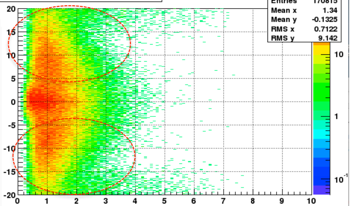
pull XY versus 1/p for No. HFT = 3
