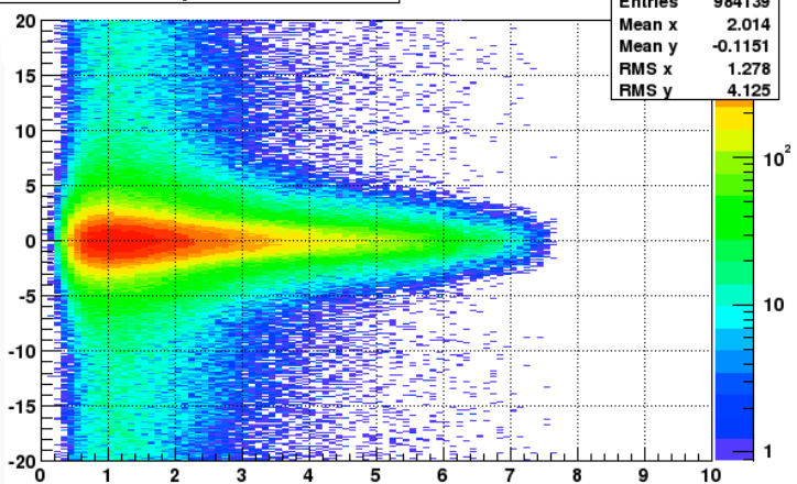
pull XY versus 1/p for No. HFT = 1
