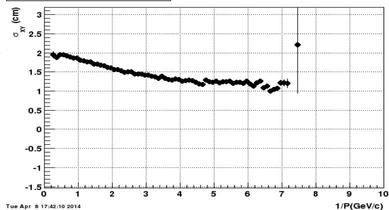
Fitted value of par[2]=Sigma
