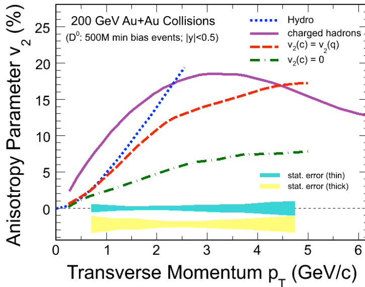
Figure 4: Elliptic flow ( v_2 ) vs p_T in Au+Au collisions at 200 GeV. The purple curve shows the measured value for charged hadrons. The red and the green curves show calculations from Ref [2] for the limiting cases that the charm quark flows like the light quarks and that the charm quark does not flow. The cyan band indicates the statistical error that can be achieved with 500 M minimum bias events for the thin detector configuration and the yellow band is for the thick configuration. In all error estimations we used the optimized cut set results.
