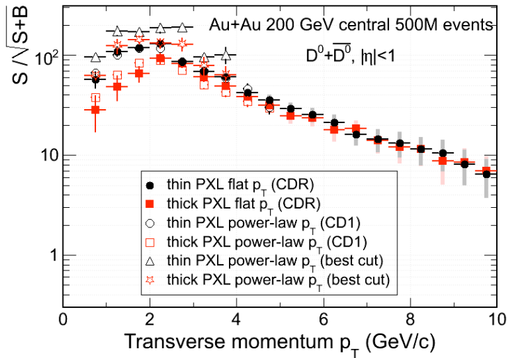
Figure 1: Signal significance as a function of p_T . Filled/open circles/squares shows the change in significance due to thickness (thin/thick) for flat/realistic spectral shape. Open triangle/stars show a new result, the signal significance for thin/thick after a careful cut optimization was performed in the lower p_T region. The gray/pink error bands (prominent only at high p_T ) are systematic uncertainties, mainly due to empty bins in the background.
