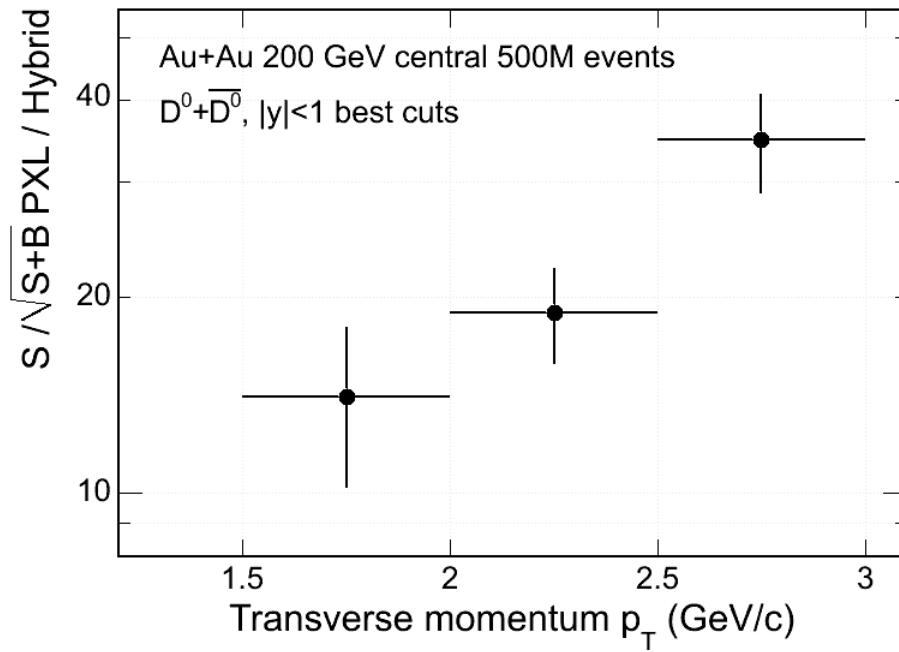
Figure 6: Gain in significance by using HFT PXL technology versus PHENIX hybrid technology.
