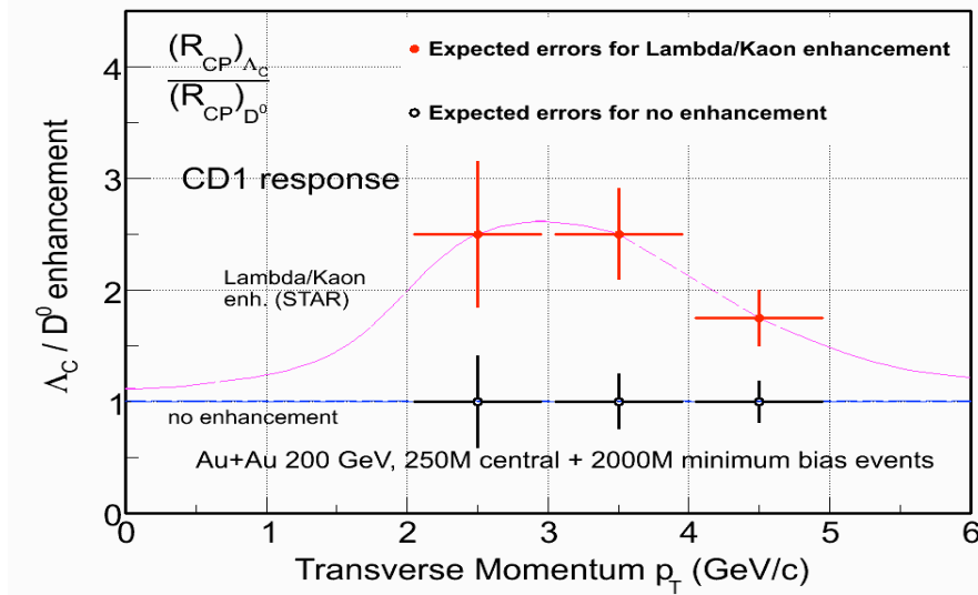
Figure 5; Expected statistical errors of the ratio of \Lambda_c to D^0 production for different assumptions about the production mechanism.
