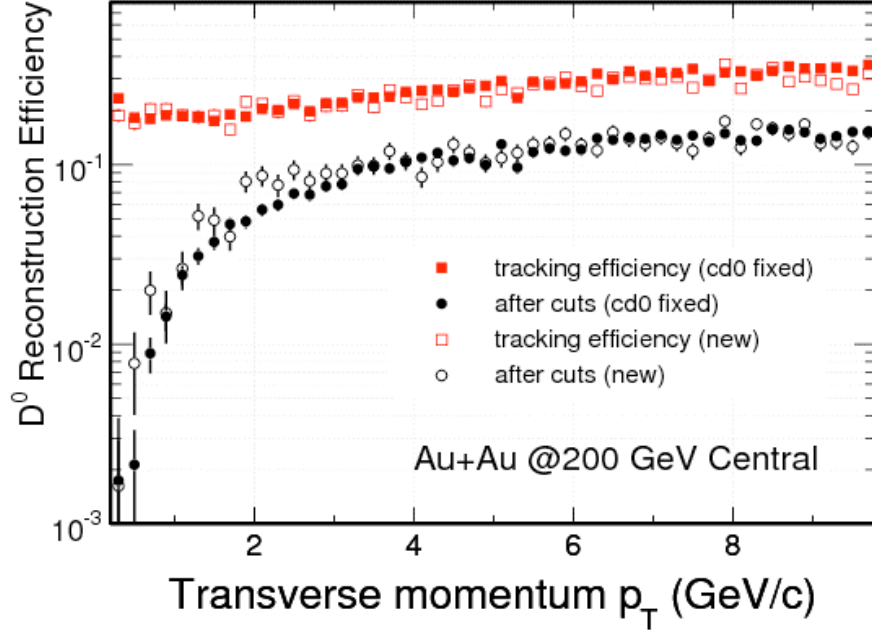
Figure 2: (Red line) Fraction of reconstructable D^0 mesons. (Black line) Fraction after a certain set of cuts has been applied to suppress background. Filled symbols are the CD0 review points and Open ones are this simulation.
