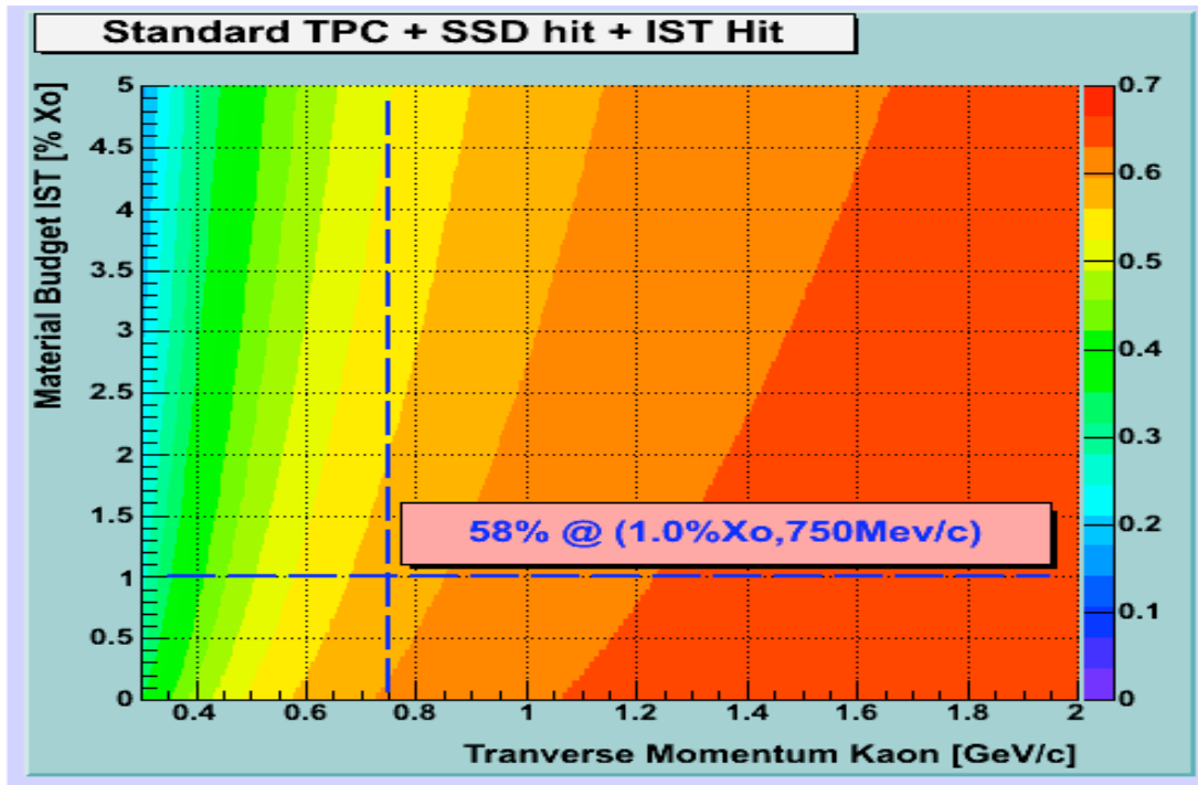
Figure 9: Fast-MC calculations for single track efficiency as a function of p_T and IST thickness.
