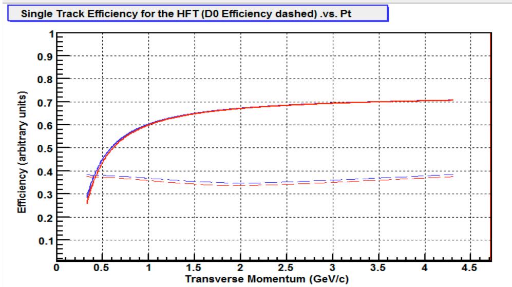
Figure 11. Impact of thicker PIXEL on single track (solid) and D0 (dashed) efficiency before cuts. The standard PIXEL is in blue and the thicker one in red.
