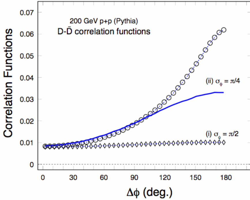
Figure 11: D-meson correlation functions for 200 GeV p+p collisions. A clear back-to-back correlation in the angular distribution of charmed mesons is observed (shown by the open circles). The solid line and the diamonds represent the results with angular smearing for \sigma_\phi of \pi/4 and \pi/2 , respectively.
